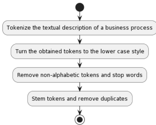
Fig. 1. The procedure for extraction of the modeling domain statements
