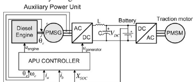
Fig. 2. Functional diagram of APU control system
