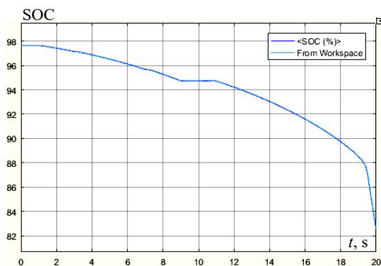
Fig. 8. Battery SOC
