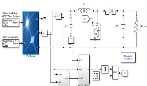
Fig. 3. Simulink PV system model
