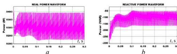
Fig. 15. Waveforms of real power ( a ) and reactive power ( b )
