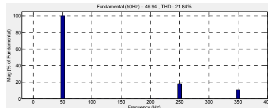
Fig. 13. Spectrum of polluted current i_{sa} without filtering
