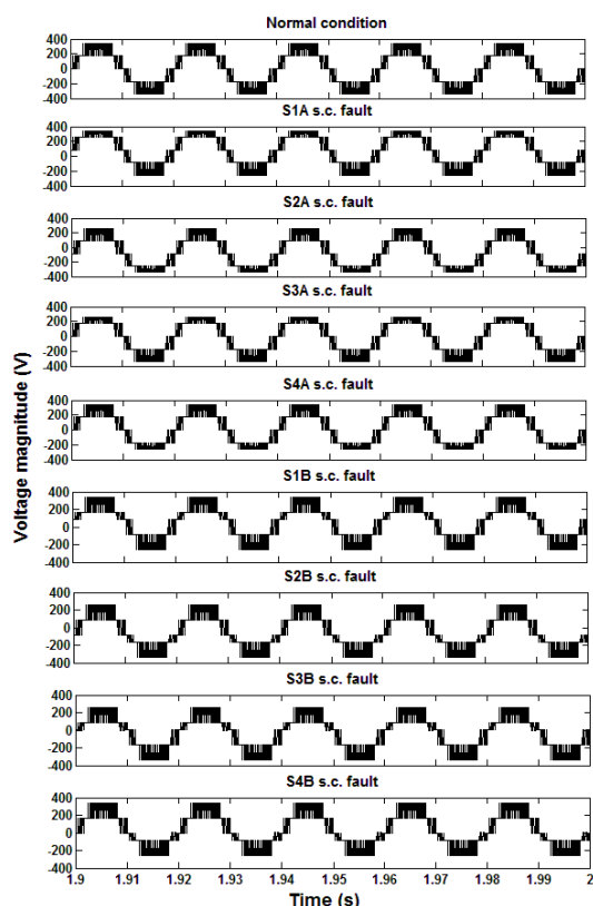
Fig. 17. Voltage output patterns in normal state as well as short circuit fault states of cells A and B
