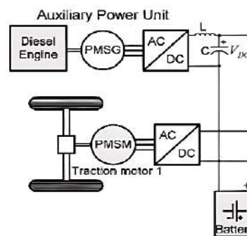
Fig. 1. Schematic diagram of series HEV drivetrain
