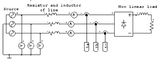
Fig. 11. Simulation model of network and polluting load without filters
