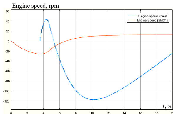
Fig. 9. Engine speed using 1-SMC and 2-SMC's
