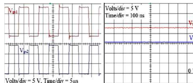
Fig. 19. Gating pulses of S1 and S2
