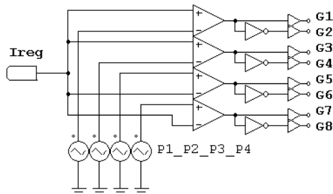
Fig. 9. PWM structure
