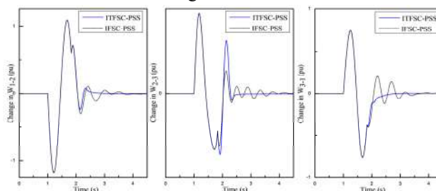
Fig. 9. Response of W_{1-2} , W_{2-3} and W_{3-1} in light operating condition
