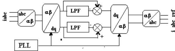
Fig. 18. Block diagram of SRF structure
