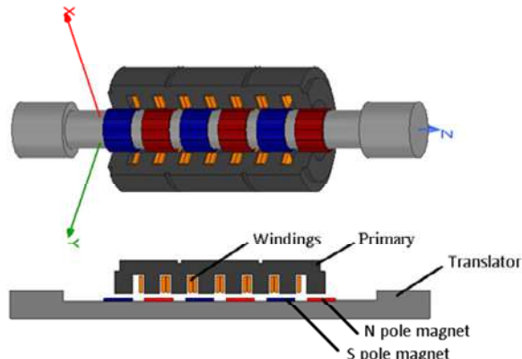
Fig. 1. 3-D and 2-D views of tube-shaped linear generator
