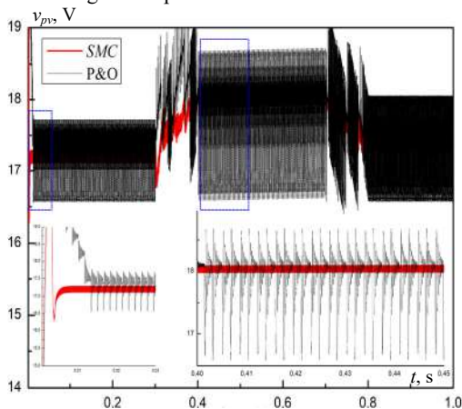
Fig. 9. PV voltage evolution for case 2
