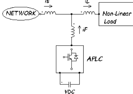
Fig. 1. Block diagram of basic APLC
