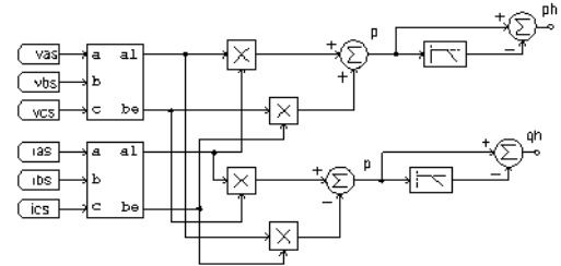
Fig. 3. Building block of calculation of harmonics powers reference
