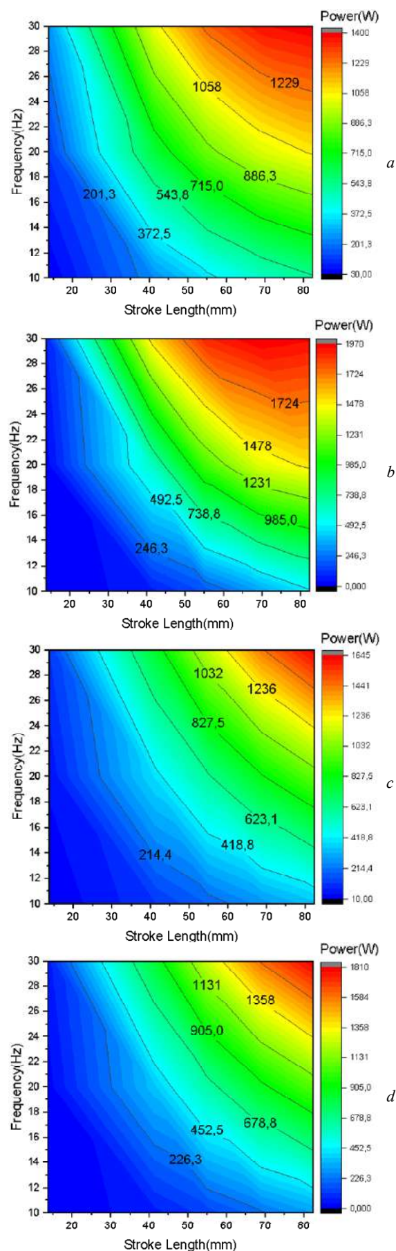
Fig. 4. Output power for stroke length and frequency: 10 \Omega (a); 10 \Omega with 100 \mu F capacitor (b); 30 \Omega (c); 30 \Omega with 100 \mu F capacitor (d)
