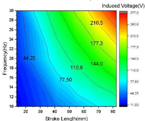
Fig. 3. Induced voltage according to stroke length and frequency in no-load condition.
