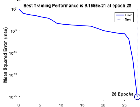
Fig. 6. Performance of the ANN
