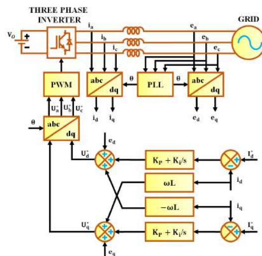
Fig. 8. A synchronous PI controller-based grid voltage synchronization
