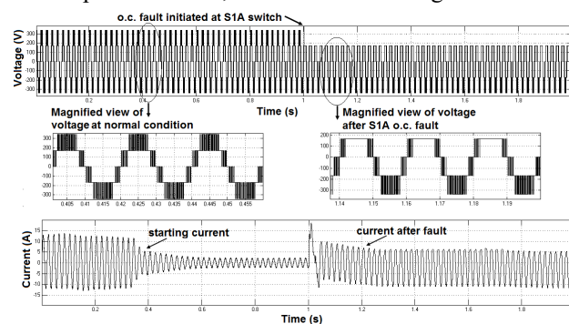
Fig. 11. Voltage and load current pattern of cascaded H-bridged inverter topology with inductive motor before and after S1A switch open circuit fault initialization
